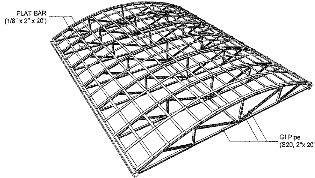
GEN-SET REHABILITATION ROOF TRUSS ISOMETRIC DETAIL SCALE: 1: 50 mm
