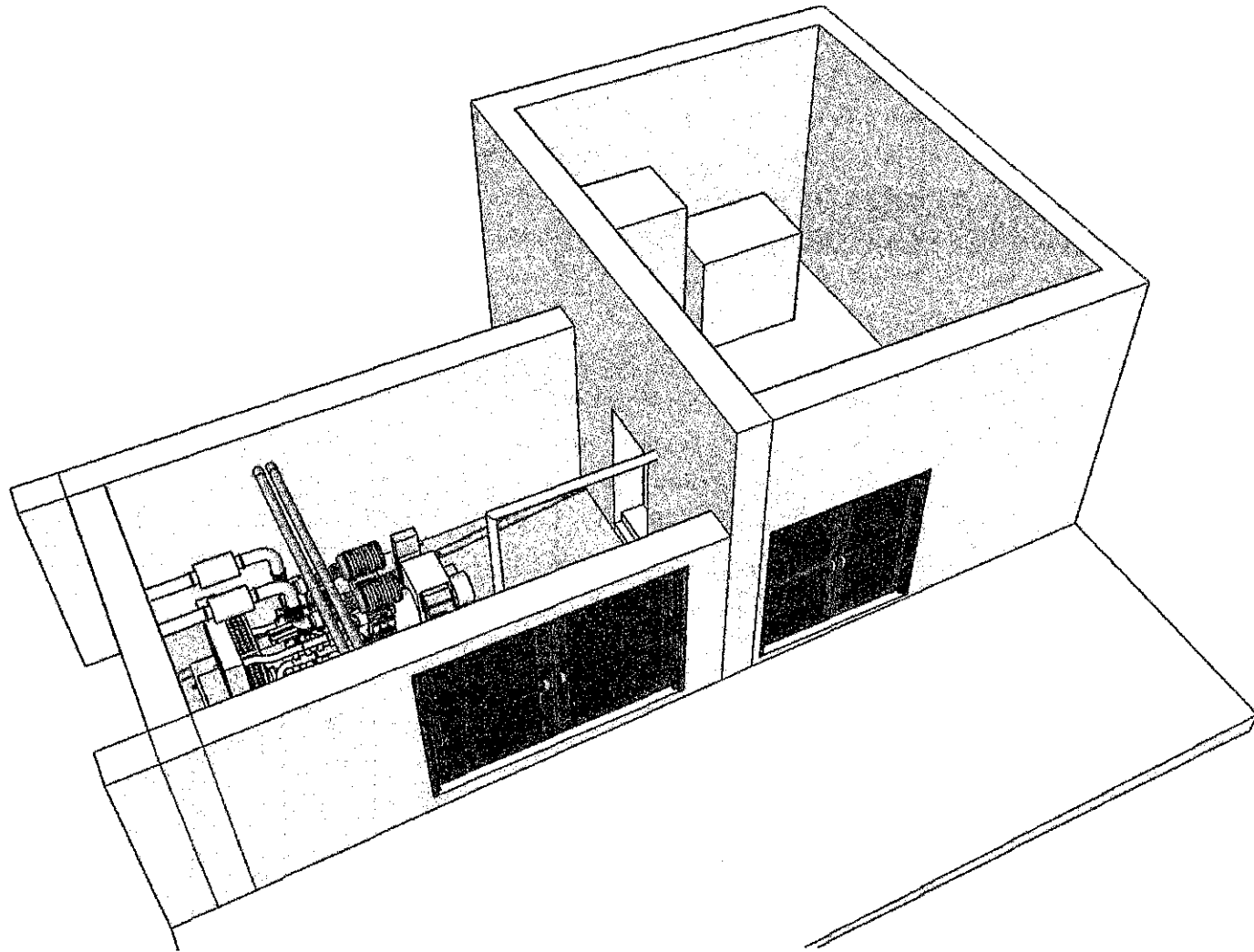
GEN-SET REHABILITATION 3D ISOMETRIC VIEW SCALE: 1:100 mm
