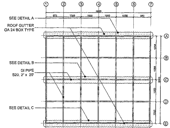
GEN-SET REHABILITATION ROOF FRAMING PLAN
