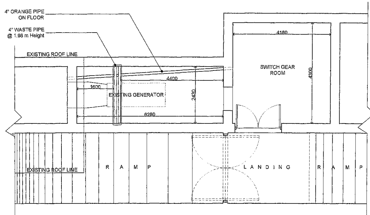
GEN-SET REHABILITATION EXISTING FLOOR PLAN SCALE: 1:100 mm
