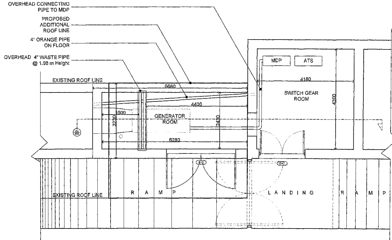
GEN-SET REHABILITATION FLOOR PLAN SCALE: 1:100 mm
