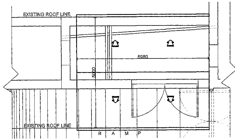
GEN-SET REHABILITATION ROOF PLAN
